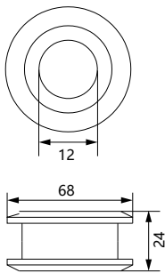
Item No: DKH03 ▪ Material: Aluminum or Stainless Steel ▪ Finish: Chrome/Brushed Nickel/Matte Black
