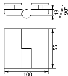
Item No: LSH32L Lift 180° Glass-to-Glass Hinge
