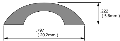
Item No: PSA01 Aluminium Threshold Seals
