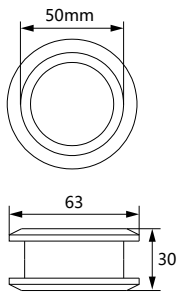
Item No: DKH04 ▪ Material: Aluminum or Stainless Steel ▪ Finish: Chrome/Brushed Nickel/Matte Black
