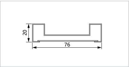
② MD3-B ▪ Side Jamb ▪ Standard Length 2200mm
