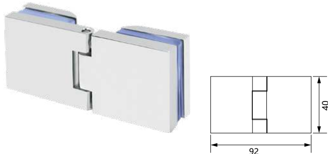
Item No: FSH062 180° Glass-to-Glass Hinge
