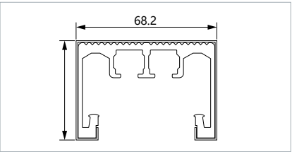
① MD3-A ▪ Header Support Bar ▪ Standard Length 1800mm
