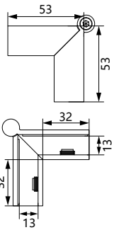
Item No: GFA Adjustable 90° to 180° Glass Clamp
