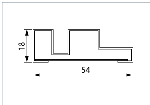
③ MD1-C ▪ Side Jamb ▪ Standard Length 2200mm
