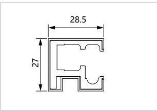
① MD1-A ▪ Header Support Bar ▪ Standard Length 2000mm
