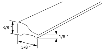
Item No: PSA03 Aluminium Threshold Seals
