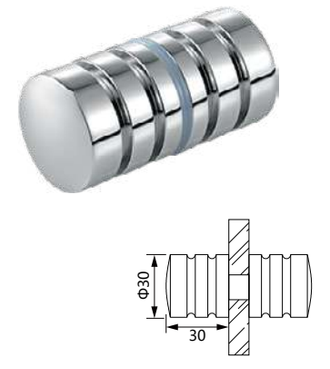
Item No: DK03 Back-to Back Knob
