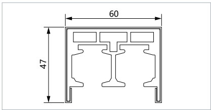
① MD2-A ▪ Header Support Bar ▪ Standard Length 1800mm
