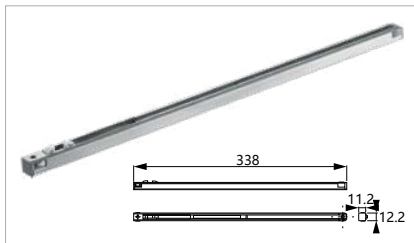
Item No: BP5 Soft-Stop Kit
