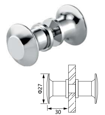
Item No: DK07 Back-to Back Knob
