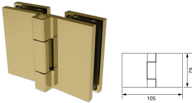
Item No: FSH052 180° Glass-to-Glass Hinge With Cover
