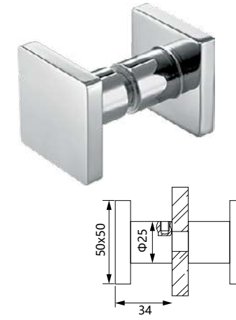
Item No: DK02 Back-to Back Knob
