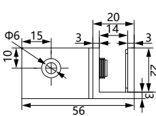
Item No: GF0L Wall Mount Glass Clamp
