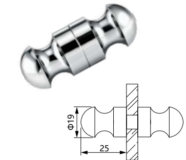
Item No: DK11 Back-to Back Knob
