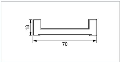
② MD2-B ▪ Side Jamb ▪ Standard Length 2200mm
