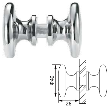
Item No: DK14 Back-to Back Knob
