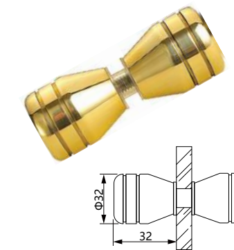
Item No: DK10 Back-to Back Knob
