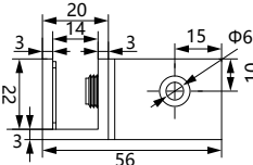
Item No: GF0R Wall Mount Glass Clamp
