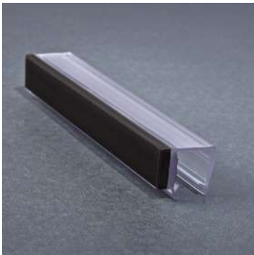
Item No: PS33 Magnetic PVC Seal ▪ Material: PVC ▪ Glass Thickness:10/12mm ▪ Finish:Clear/white/Matte Black
