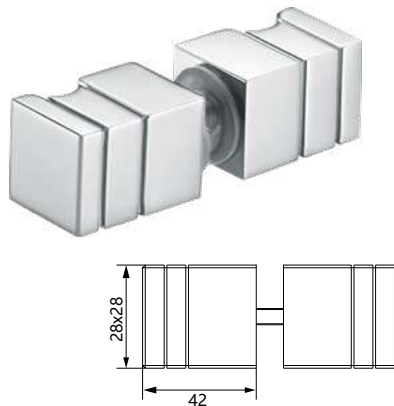
Item No: DK17 Back-to Back Knob
