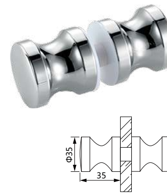
Item No: DK05 Back-to Back Knob
