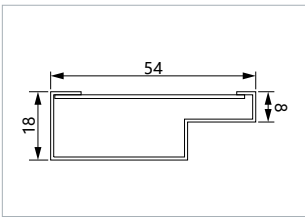
② MD1-B ▪ Side Jamb ▪ Standard Length 2200mm
