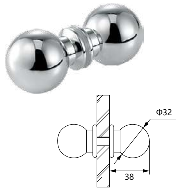
Item No: DK18 Back-to Back Knob
