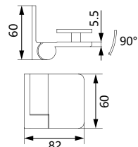
Item No: LSH14L Lift Wall Mount Hinge
