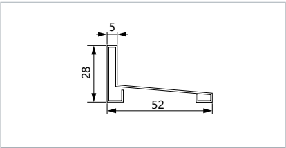
③ MD3-C ▪ Bottom Sill
