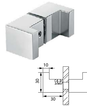
Item No: DK01 Back-to Back Knob
